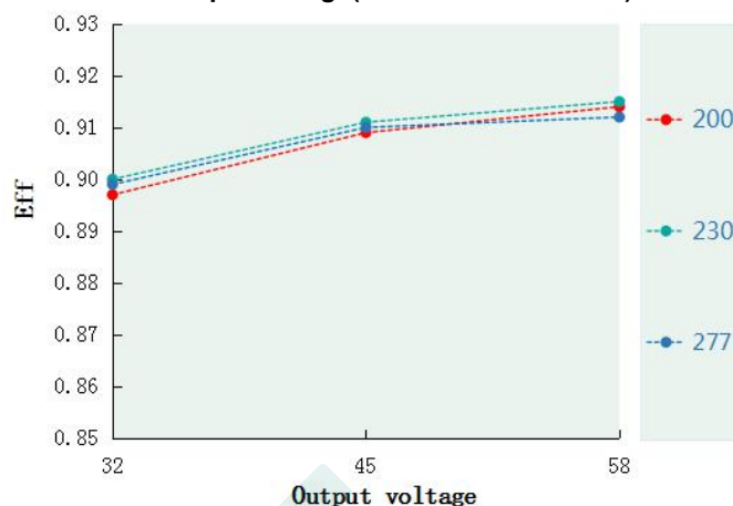
Eff. VS Output voltage(DL-100I-V58P/A-MAS)
