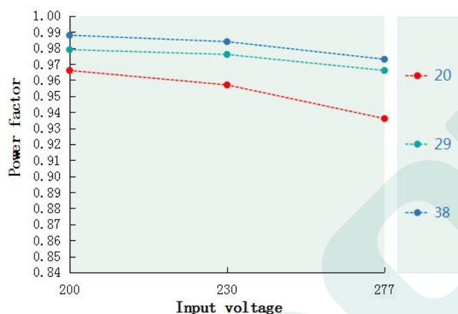
Power factor VS Input voltage(DL-100I-V38P/A-MAS)
