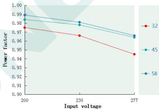
Power factor VS Input voltage(DL-100I-V58P/A-MAS)
