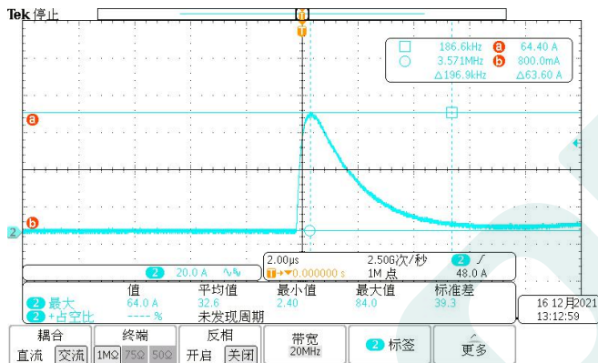
Inrush Current(DL-100I-A/P-MAS)
