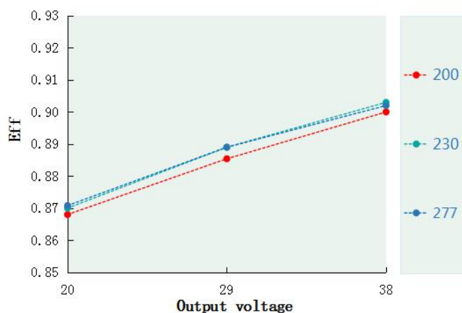
Eff. VS Output voltage(DL-100I-V38P/A-MAS)
