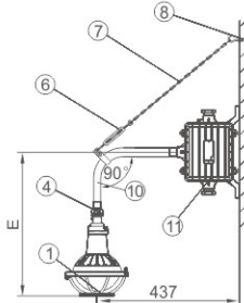
壁式90° (b2)/Wall type90° (b2)
