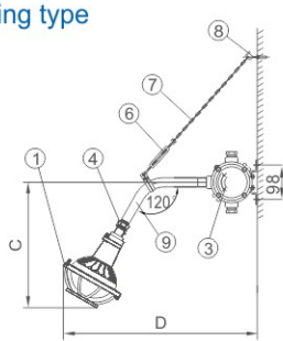
壁式30° (b1) Wall type30° (b1)
