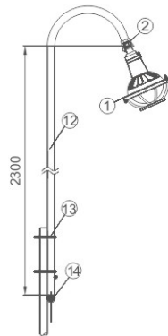
护栏式2(h2)/Fence type2(h2)
