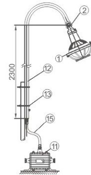
护栏式1(h1) Fence type1(h1)
