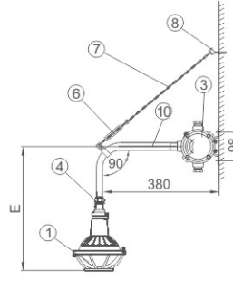
壁式90° (b2) Wall type90° (b2)
