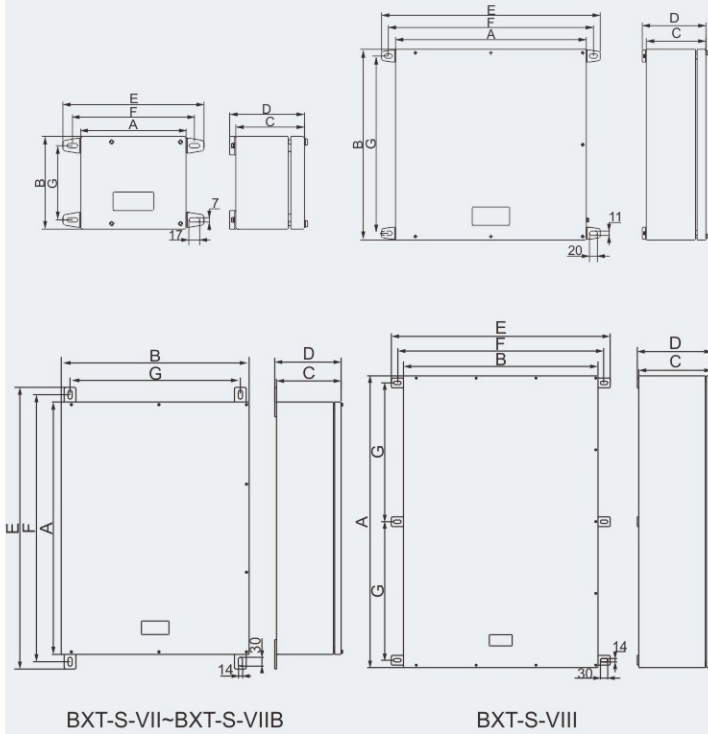
Selection table of BXT-S series increased safety enclosures (all dimensions in mm)
