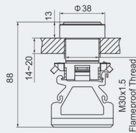
M30x1.5 Flameproof Thread Pushbutton with indicator
